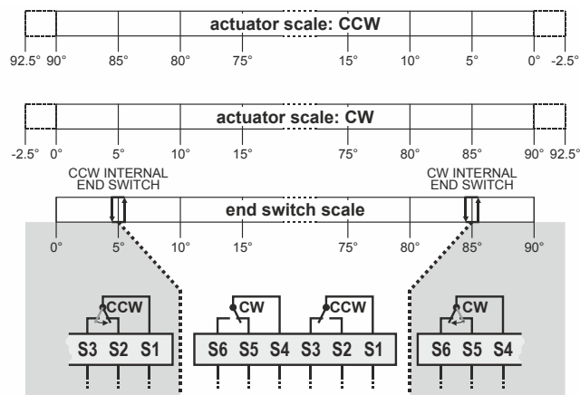
Fig. 7. Internal end switch triggering points
