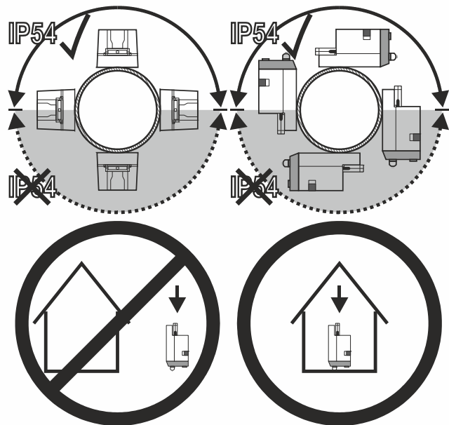
Fig. 8. Mounting for IP54
