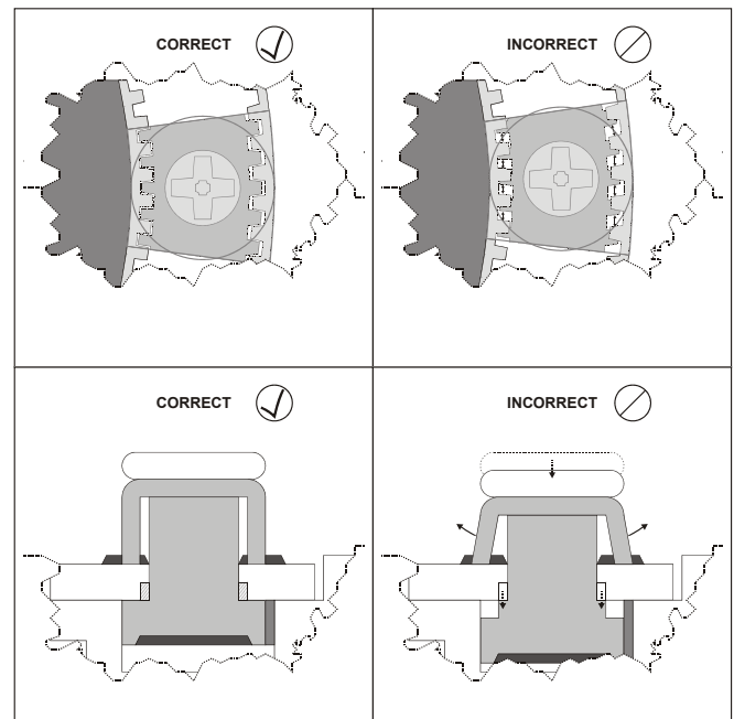
Fig. 6. Correct / incorrect tightening of end limits
