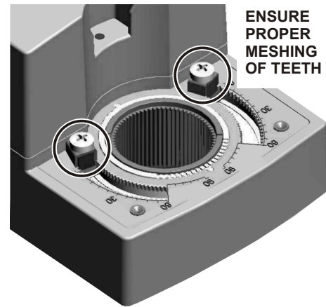
Fig. 5. Mechanical end limits
